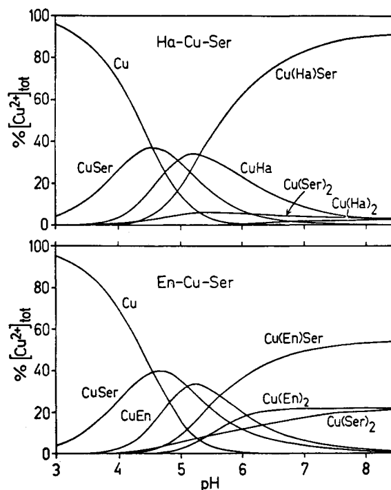
Figure 10. Relative concentrations of complex species as per cent of total Cu(II) in aqueous solution containing 10^{-3} M total Cu(II) and each of two ligands over a range of pH at 37^\circ . Upper figure: histamine (Ha) and serine (Ser) ligands. Lower figure: diaminoethane (en) and serine ligands. The possibility of hydrolysis at high pH was omitted from the calculations. Figure is from ref 182 and is based on equilibrium constants presented by D. D. Perrin, I. G. Sayce, and V. S. Sharma, J. Chem. Soc. A , 1755 (1967).
