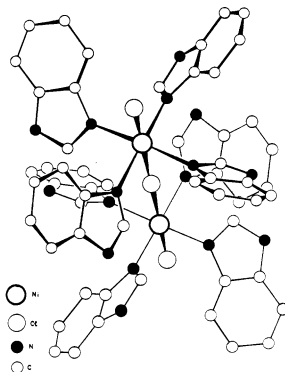
Figure 3. The [\text{Ni}_2(\text{BzIm})_8\text{Cl}_3]^+ unit in \mu -chloro-bis(chlorotetra-benzimidazole)nickel(II) chloride. Reproduced from ref 107.
