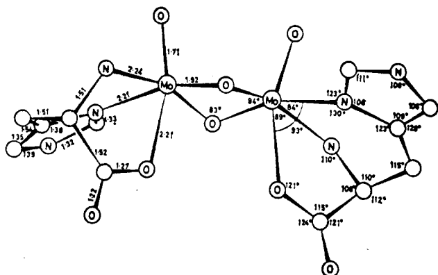
Figure 8. Molecular structure of \text{Mo}_2\text{O}_4(\text{L-histidine})_2 . Reproduced from ref 169.
